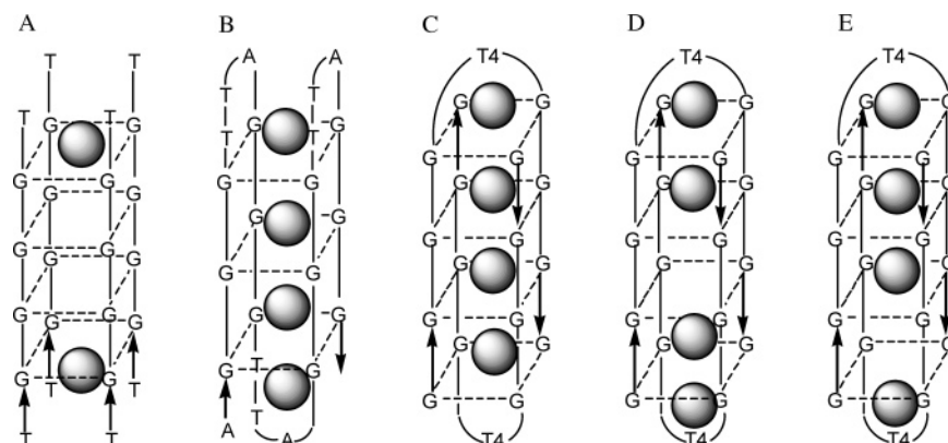
FIGURE 9: Proposed binding modes of \text{H}_2\text{TMPyP4} to G-quadruplexes. (A) Two \text{H}_2\text{TMPyP4} molecules are externally stacked at the opposite end of (\text{TG}_4\text{T})_4 . (B) Two \text{H}_2\text{TMPyP4} molecules are intercalated in the diagonal and lateral loops, and the other two \text{H}_2\text{TMPyP4} are intercalated in the two intervals between adjacent G-tetrads of \text{AG}_3(\text{T}_2\text{AG}_3)_3 . (C) One \text{H}_2\text{TMPyP4} molecule binds to one of the T4 loop regions, and the other three \text{H}_2\text{TMPyP4} molecules intercalate the three intervals between adjacent G-tetrads of (\text{G}_4\text{T}_4\text{G}_4)_2 G-quadruplexes. (D and E) Two \text{H}_2\text{TMPyP4} molecules stack in the two T4 loops, and the other two molecules bind to the two of three intervals of (\text{G}_4\text{T}_4\text{G}_4)_2 G-quadruplexes. Balls denote the \text{H}_2\text{TMPyP4} molecules, and arrows denote 5' \rightarrow 3' strand alignment for each DNA.
